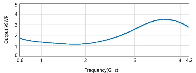
Output VSWR vs. Frequency
