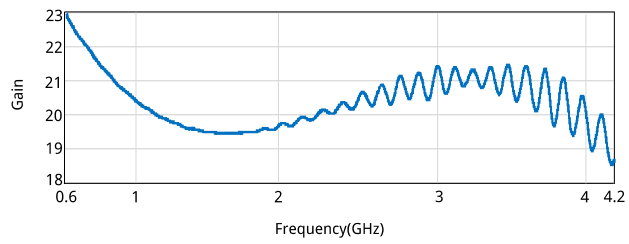
Gain vs. Frequency
