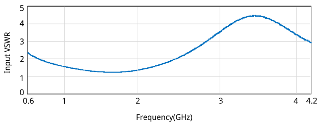
Input VSWR vs. Frequency
